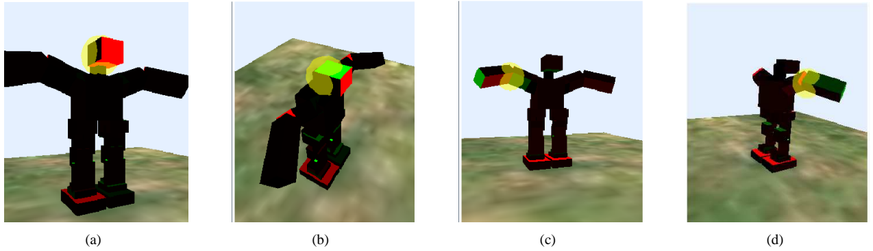
Fig. 6. The importance of each of the sensors in determining the variation of the head orientation ((a) and (b), joint 1 of Fig. 3(b)) and the variation of the elbow joint angle((c) and (d), joint 7 of Fig. 3). The various sensors are colored red or green depending on the sign of the relative coefficient, while its absolute value is represented by the intensity of color. A yellow sphere highlights the position of the joint which depends on the coefficients used to color the sensors.
