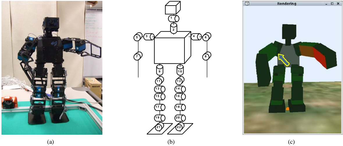
Fig. 3. (a) A photo of the VStone VisiON 4G humanoid robot, (b) a schematic of its joints, and (c) the 3D rendered model, where the left upper arm and forearm have just been pushed. The 3D model display also shows the projection of the center of gravity onto the ground (represented by an orange sphere) and its velocity (a blue arrow, in this figure surrounded by a yellow border to make it more easily visible to the reader) which can be useful to expert users in motion development.
